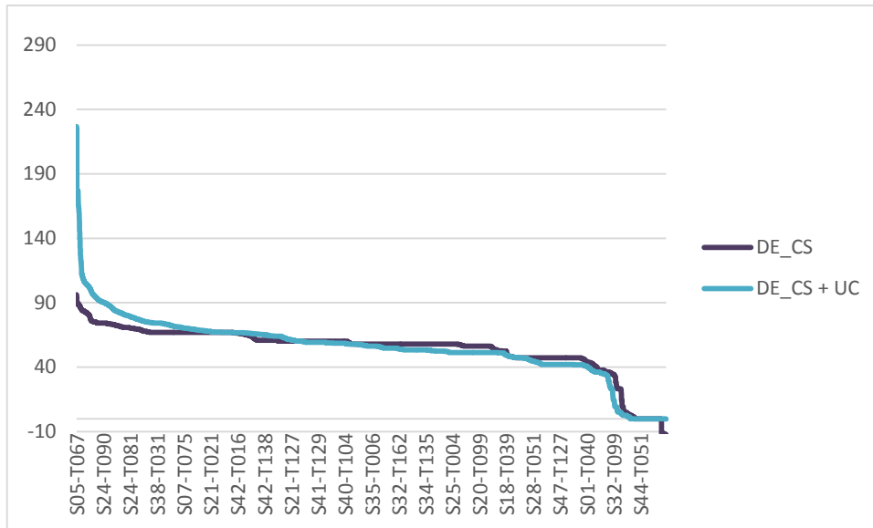
Figure 28: Duration curve for electricity prices in central South Germany, with and without UC. (The light blue line represents prices with UC)
