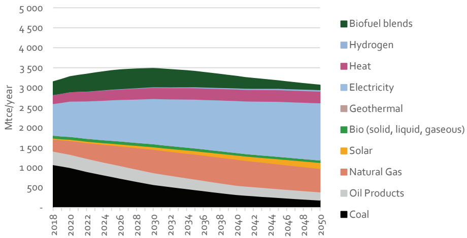
Figure 10-1: The development of final energy consumption (Mtce) by energy type from 2018-2050 in the Stated Policies scenario
